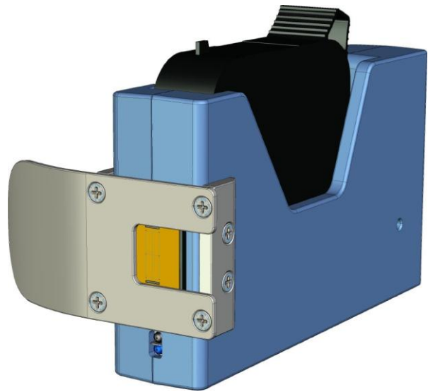
Anti-shock plate installation
