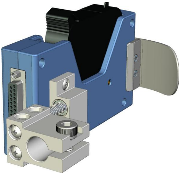
Springback mechanism installation
